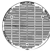
Type M1 ADA Grate Approx. 639 sq. in. open area
